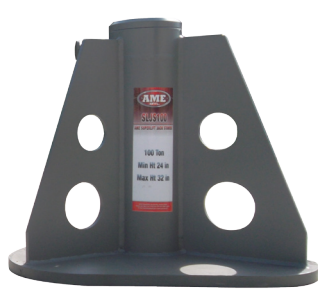
High Tonnage Jack Stands
